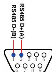
For RS485 Mode
